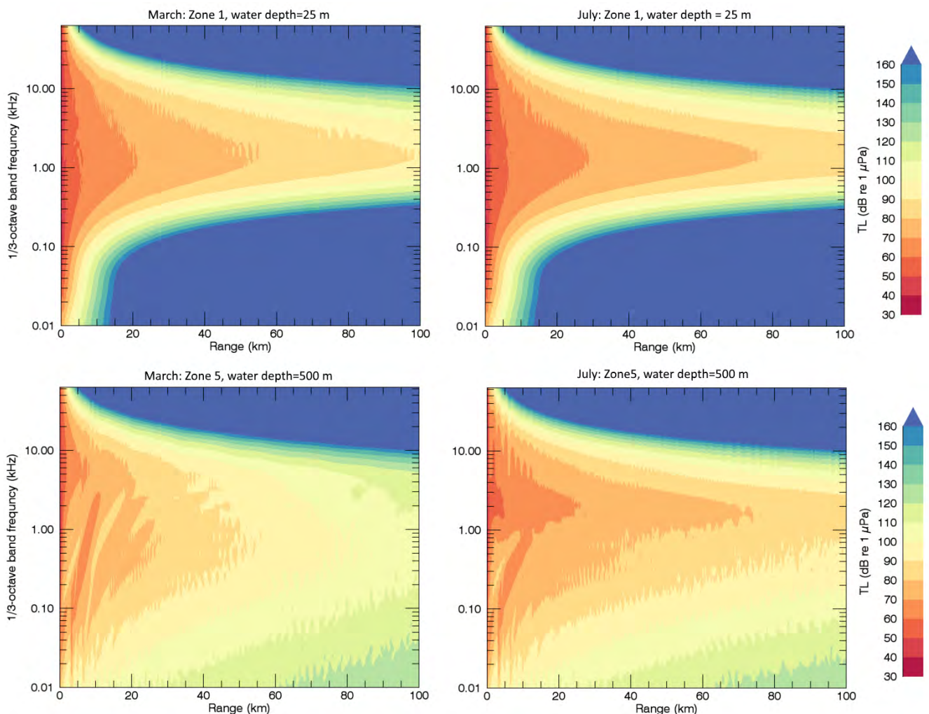
Figure B-2: Example plots of modelled transmission loss as a function of distance from the source and frequency. This example represents the transmission loss in Zone 1 (top) and Zone 5 (bottom) seen in Figure B-1, for March (left) and July (right). Source and receiver depths are 7 and 10 m, respectively.
