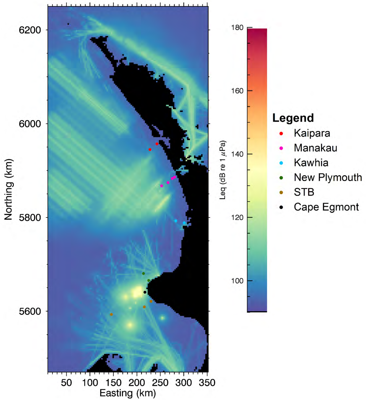
Figure 9: One-month equivalent continuous underwater noise levels ( L_{eq} ) for March: Broadband SPL.
