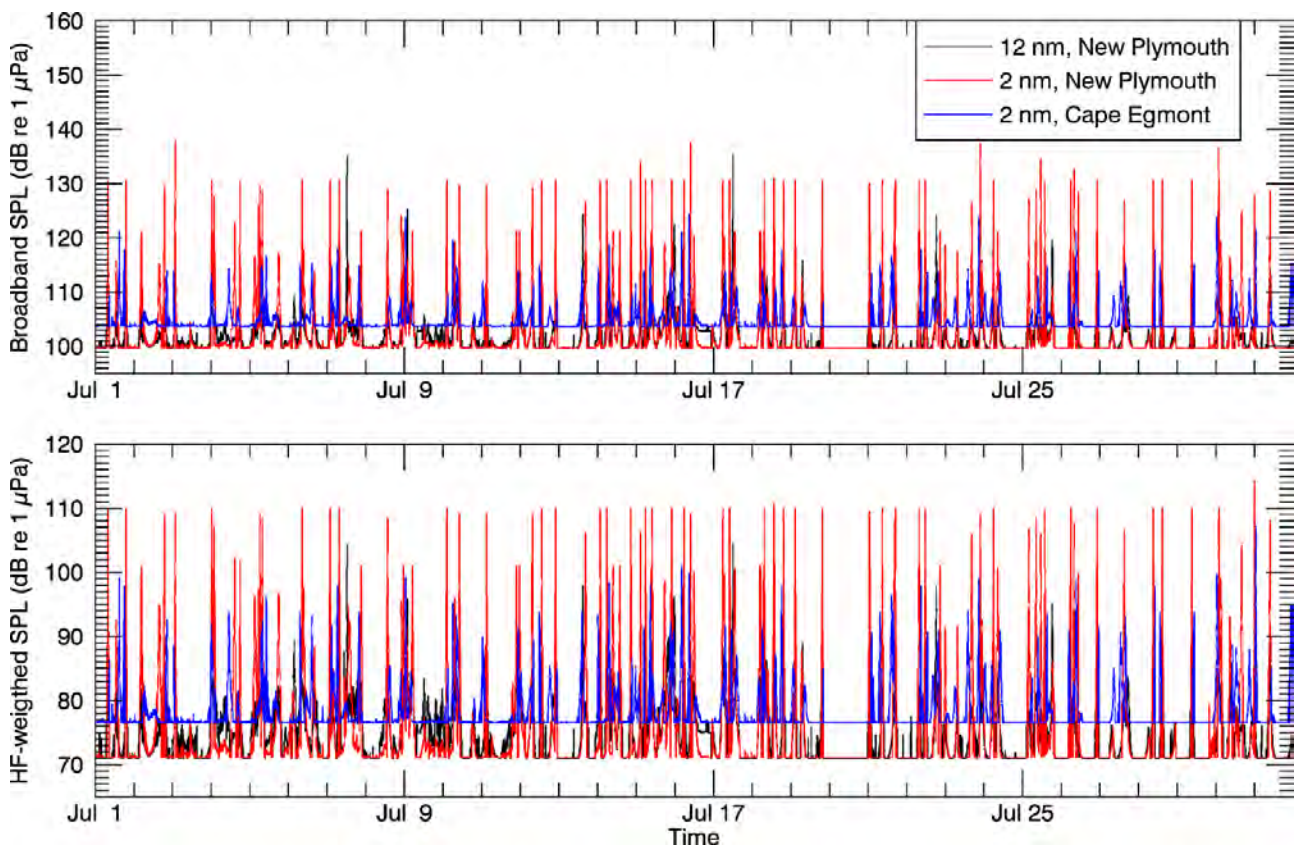
Figure 26: New Plymouth and Cape Egmont, July: SPL variation over time, broadband SPL (top) and HF-weighted SPL (bottom). Locations provided in Figure 1 and Table 1.
