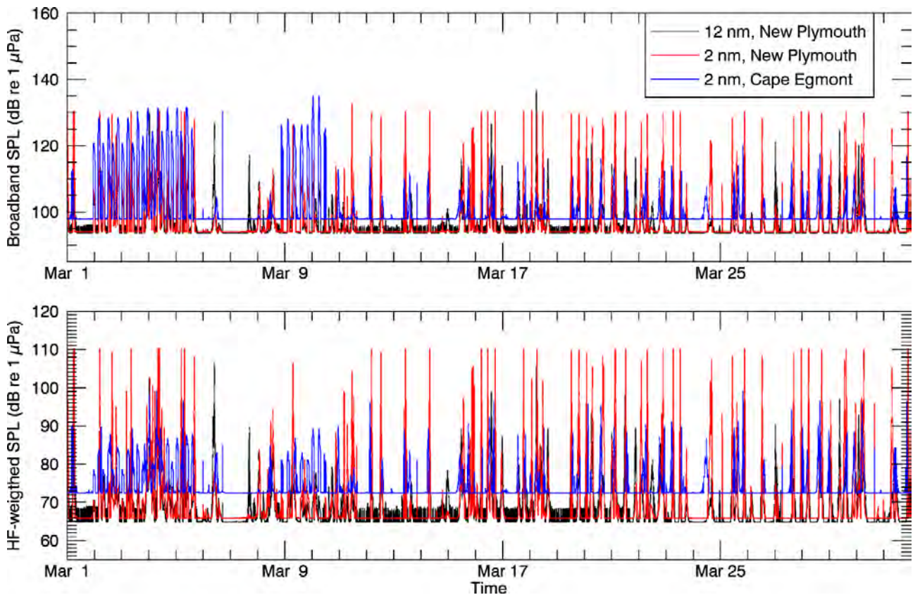
Figure 16: New Plymouth and Cape Egmont, March: SPL variation over time, broadband SPL (top) and HF-weighted SPL (bottom). Locations provided in Figure 1 and Table 1.
