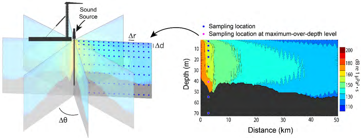
Figure E-4. Modeled three-dimensional sound field (N \times 2-D method) and maximum-over-depth modeling approach. Sampling locations are shown as blue dots on both figures. On the right panel, the pink dot represents the sampling location where the sound level is maximum over the water column. This maximum-over-depth level is used in calculating distances to sound level thresholds for some marine animals.
